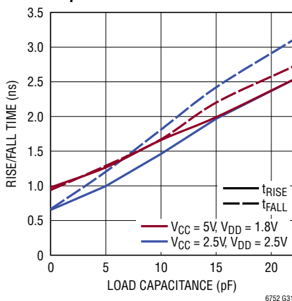
Rise/Fall times vs Capacitive Load
