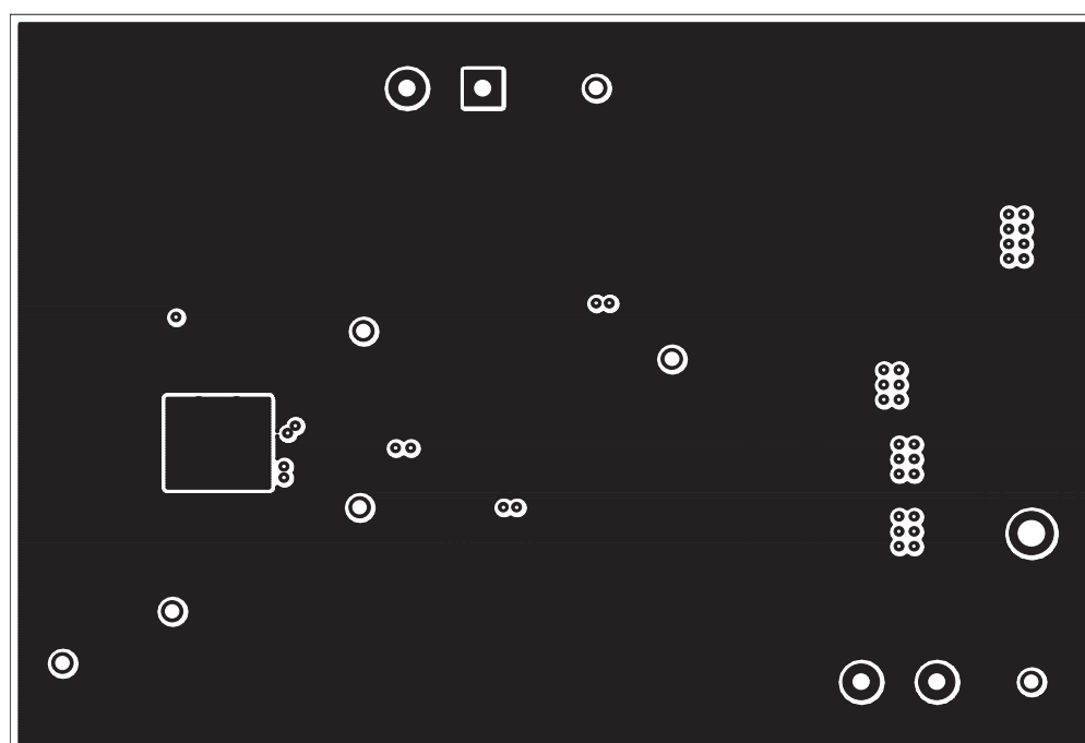
Figure 25. Bottom Layer Copper
