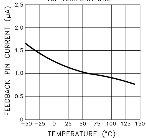
FEEDBACK PIN BIAS CURRENT vs. TEMPERATURE
