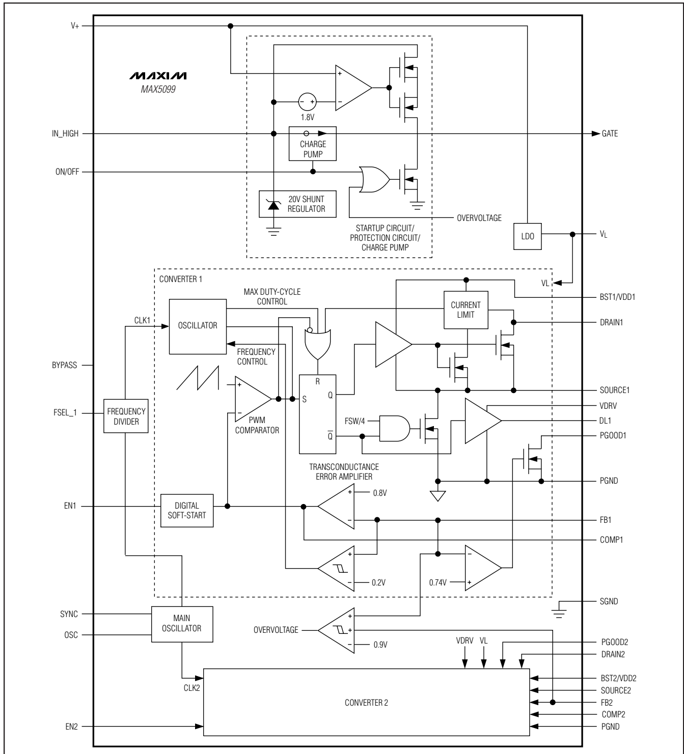
Functional Diagram
