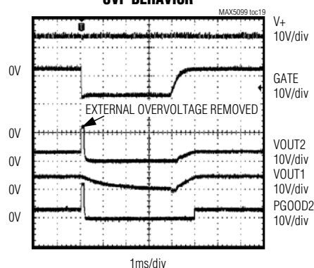
OVP BEHAVIOR
