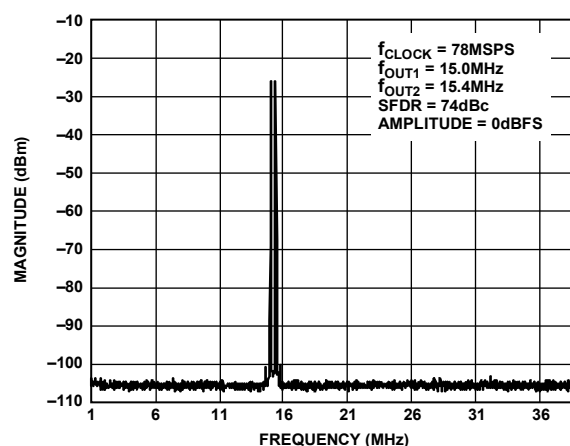
Figure 42. Dual-Tone SFDR
