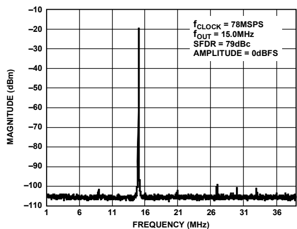
Figure 41. Single-Tone SFDR
