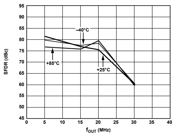
Figure 40. SFDR vs. Temperature at 80 MSPS
