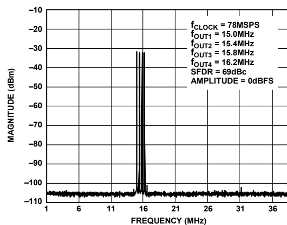
Figure 43. Four-Tone SFDR
