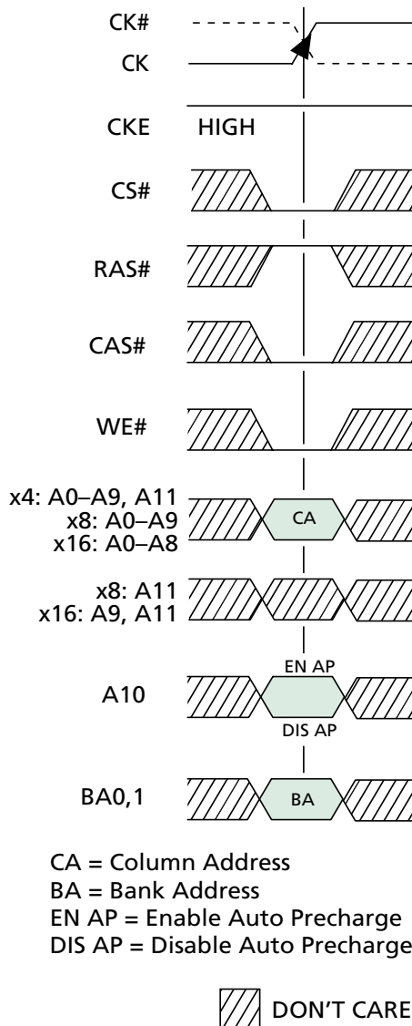
Figure 14 WRITE Command
