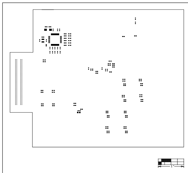
MAX1153/MAX11254 Family EV Kit—Bottom Paste
