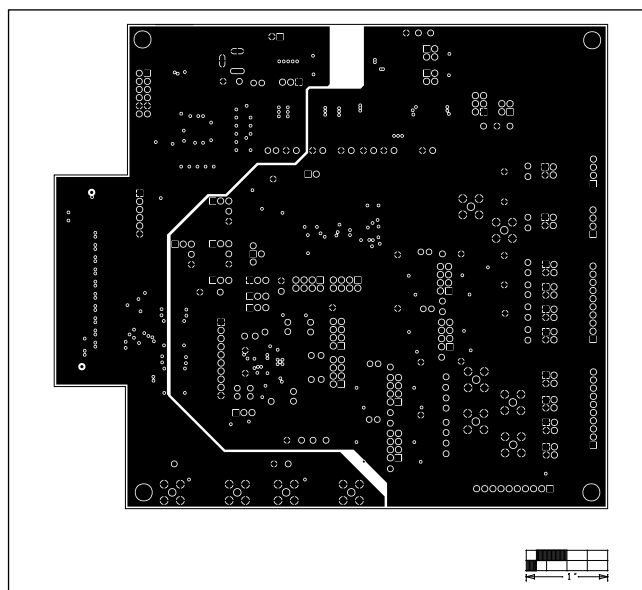
MAX1153/MAX11254 Family EV Kit—Internal 5
