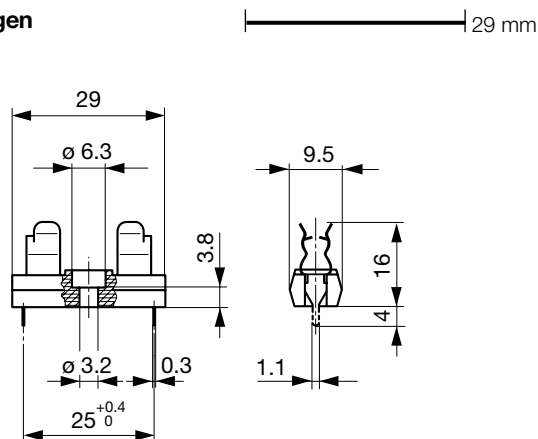
Drilling diagram
