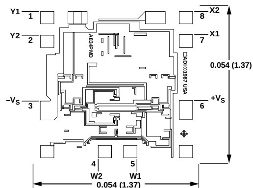
Figure 2. Metallization Photograph
