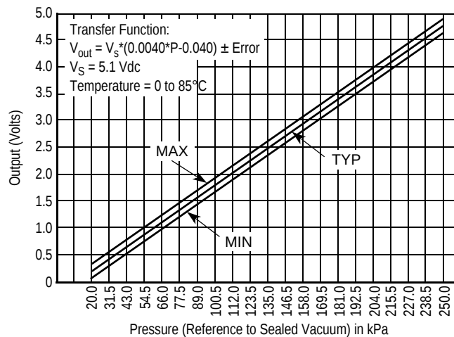
Figure 4. Output vs. Absolute Pressure
