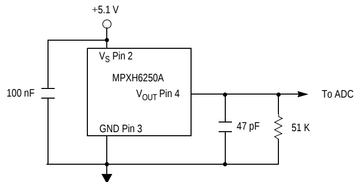
Figure 3. Typical Application Circuit (Output Source Current Operation)
