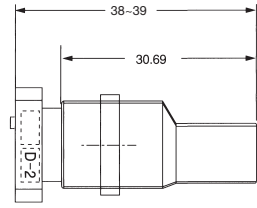
Panel/Free-Hanging Type
