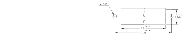
Panel Cutout
