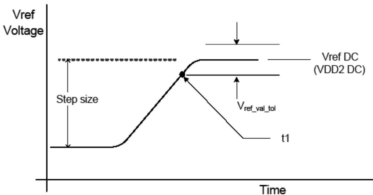
VREF step single stepsize increment case
