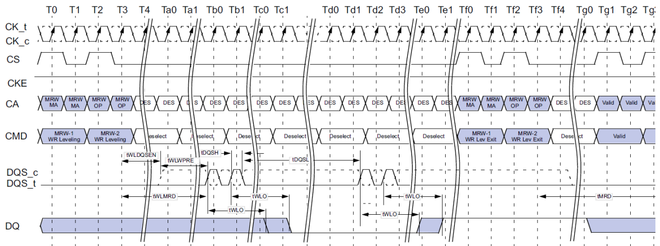
Write Leveling Timing, tDQSL(max)
