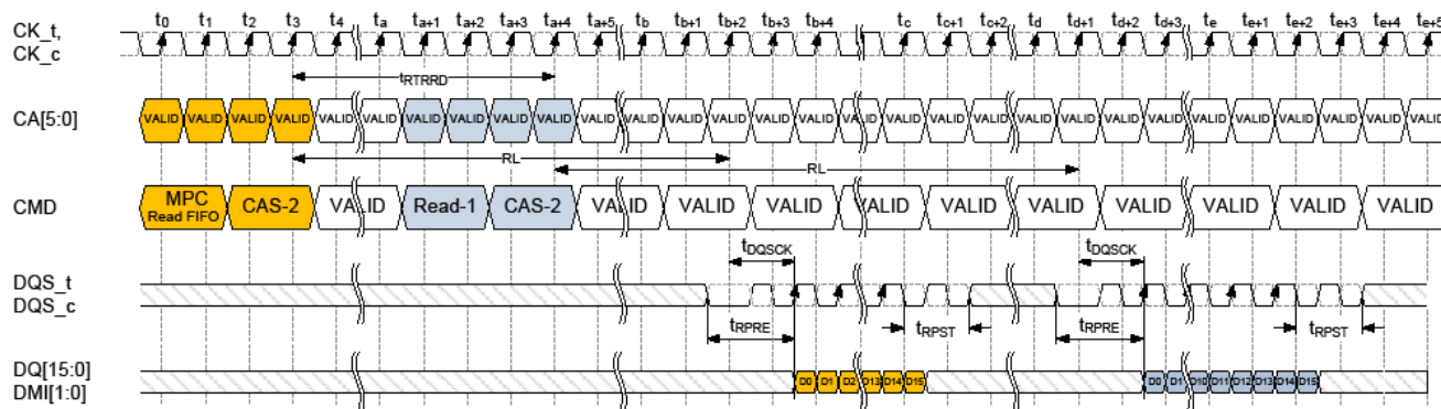
MPC [RD FIFO] Operation : tRPRE=toggling, tRPST=1.5nCK
