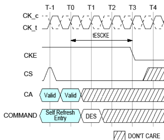
tESCKE Timing
