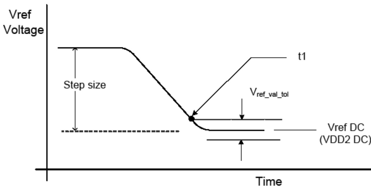
VREF step single stepsize decrement case
