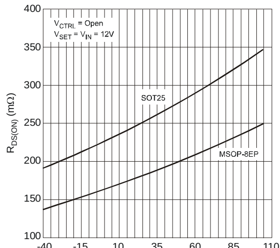
Figure 6 SW R_{DS(ON)} vs. Temperature
