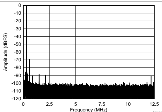
SFDR = 68 dBc, SNR = 66.7 dBFS, SINAD = 66.5 dBFS, THD = 92 dBc, HD2 = 68 dBc, HD3 = 90 dBc, SFDR = 91 dBc (non 23)
