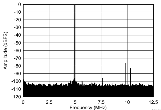
SFDR = 76 dBc, SNR = 69.4 dBFS, SINAD = 68.8 dBFS, THD = 75 dBc, HD2 = 76 dBc, HD3 = 83 dBc, SFDR = 96 dBc (non 23)
