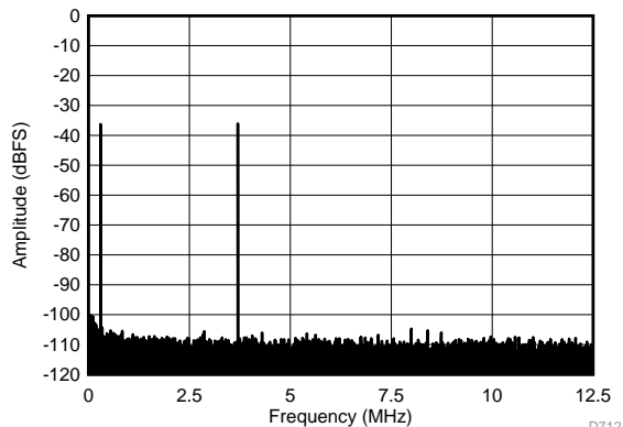
f_{IN1} = 46.3\text{ MHz} , f_{IN2} = 50.3\text{ MHz} , IMD3 = 105 dBFS, each tone at -36 dBFS
