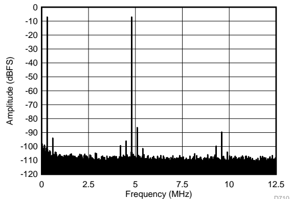
f_{IN1} = 46.3\text{ MHz} , f_{IN2} = 50.3\text{ MHz} , IMD3 = 86 dBFS, each tone at -7 dBFS
