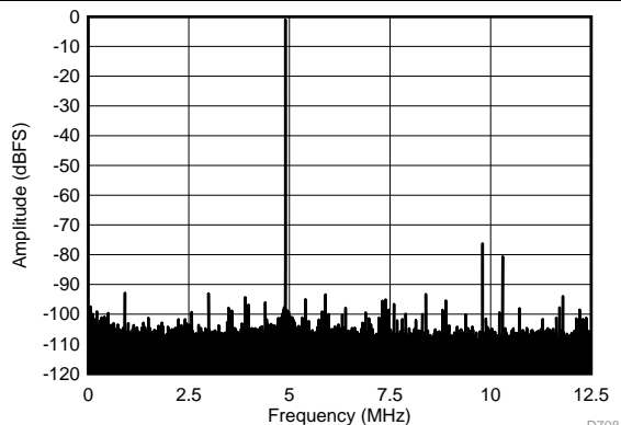
SFDR = 75 dBc, SNR = 69.6 dBFS, SINAD = 68.6 dBFS, THD = 74 dBc, HD2 = 75 dBc, HD3 = 80 dBc, SFDR = 91 dBc (non 23)
