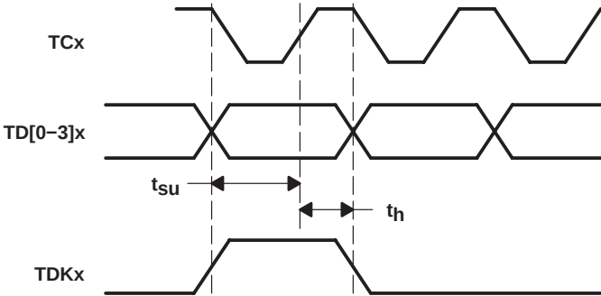
Figure 2. Transmit Timing Waveform
