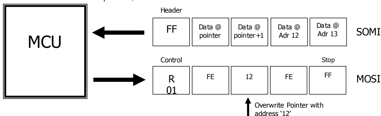
Figure 6.3 SPI Read
