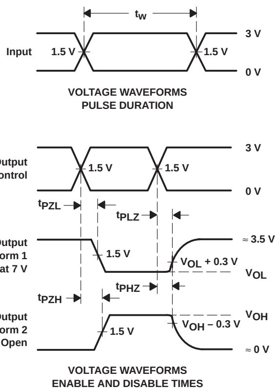
Figure 10. Load Circuit and Voltage Waveforms
