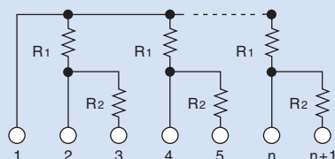
E circuit
