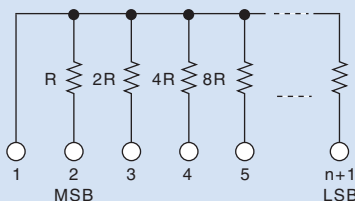
K circuit
