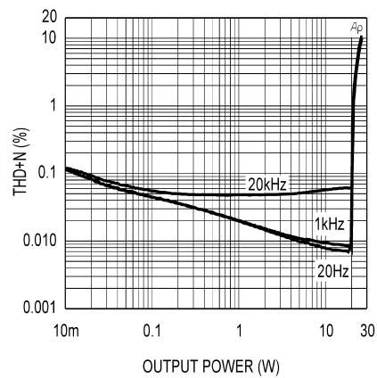
THD+N vs Output Power \pm 22\text{V} , R_L = 8\Omega , 80kHz BW
