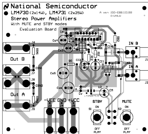
Composite View
