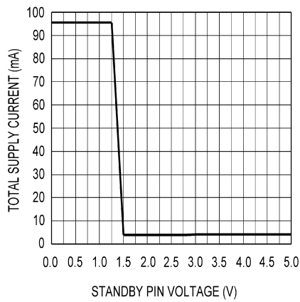
Supply Current vs Standby Pin Voltage \pm 22\text{V}
