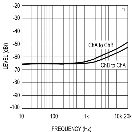
Crosstalk vs Frequency \pm 18\text{V} , P_O = 10\text{W} , R_L = 4\Omega , 80kHz BW
