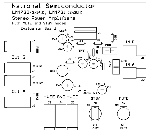
Silk Screen
