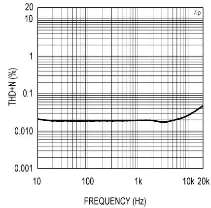
THD+N vs Frequency \pm 22\text{V} , P_O = 1\text{W/Channel} , R_L = 8\Omega , 80kHz BW
