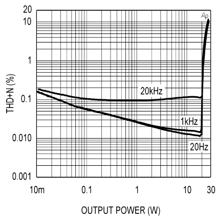
THD+N vs Output Power \pm 18\text{V} , R_L = 4\Omega , 80kHz BW
