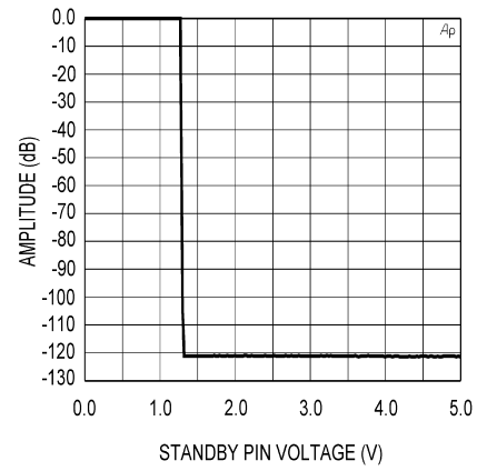
Standby Attenuation vs Standby Pin Voltage \pm 22\text{V} , P_O = 1\text{W} , R_L = 8\Omega , 80kHz BW
