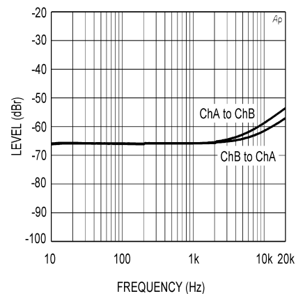
Crosstalk vs Frequency \pm 22\text{V} , P_O = 10\text{W} , R_L = 8\Omega , 80kHz BW
