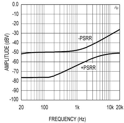
PSRR vs Frequency \pm 22\text{V} , V_{\text{RIPPLE}} = 1\text{V}_{\text{RMS}} , R_L = 8\Omega , 80kHz BW
