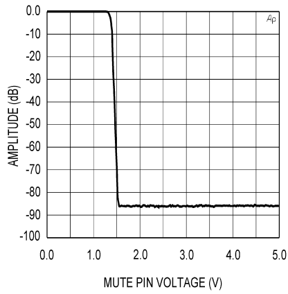
Mute Attenuation vs Mute Pin Voltage \pm 22\text{V} , P_O = 1\text{W} , R_L = 8\Omega , 80kHz BW
