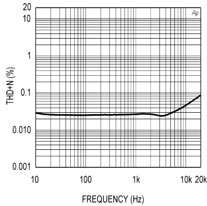
THD+N vs Frequency \pm 18\text{V} , P_O = 1\text{W/Channel} , R_L = 4\Omega , 80kHz BW
