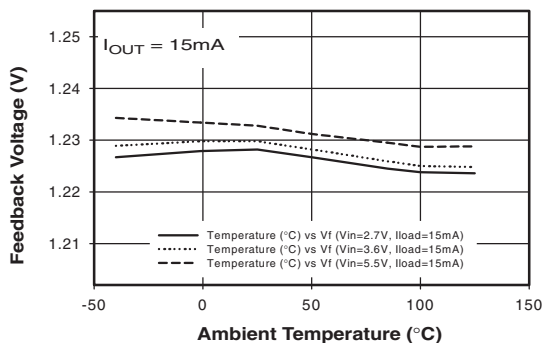
Feedback Voltage vs Ambient Temperature
