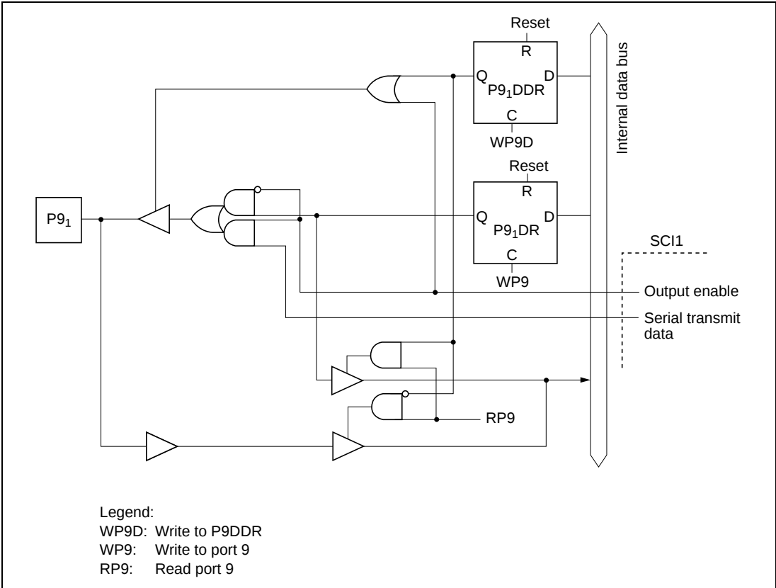
Figure C.8 (b) Port 9 Block Diagram (Pin P9 1 )
