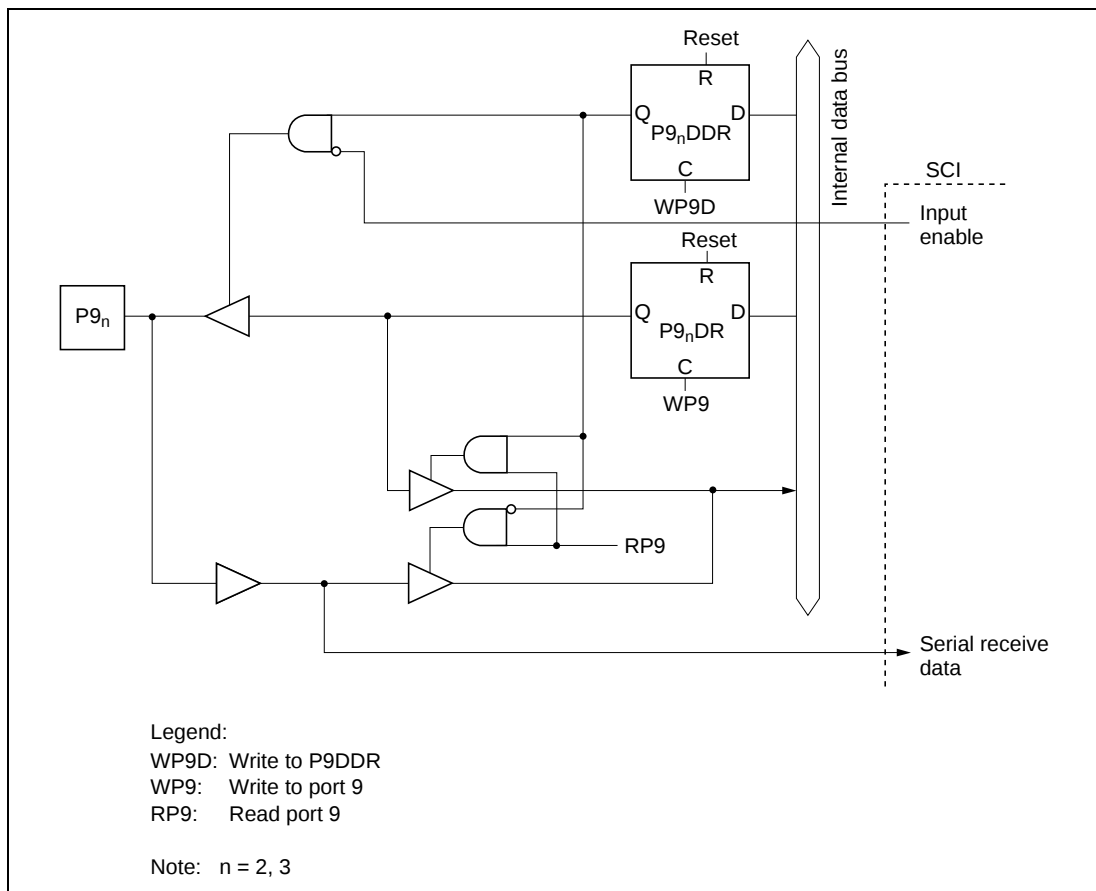
Figure C.8 (c) Port 9 Block Diagram (Pin P9 n , P9 i )
