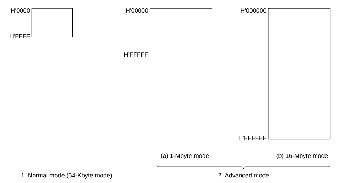
Figure 2.2 Memory Map
