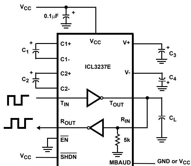
FIGURE 5. TRANSMITTER LOOPBACK TEST CIRCUIT
