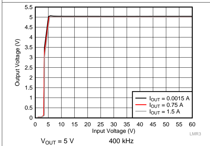
Figure 24. Line Regulation
