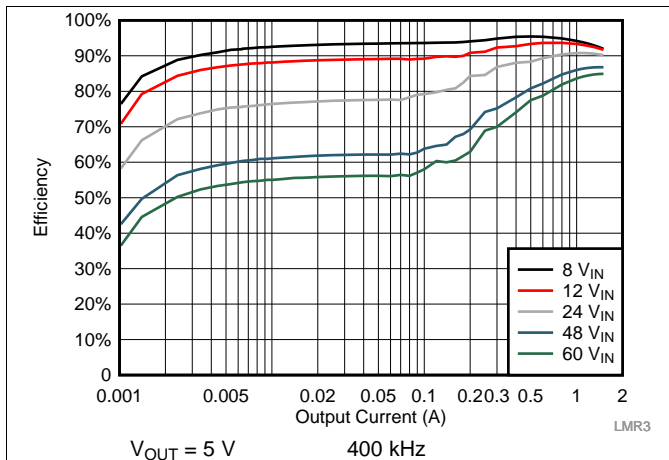
Figure 20. Efficiency
