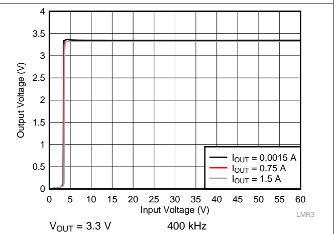
Figure 25. Line Regulation
