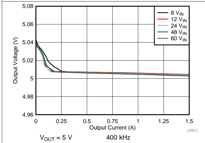
Figure 22. Load Regulation
