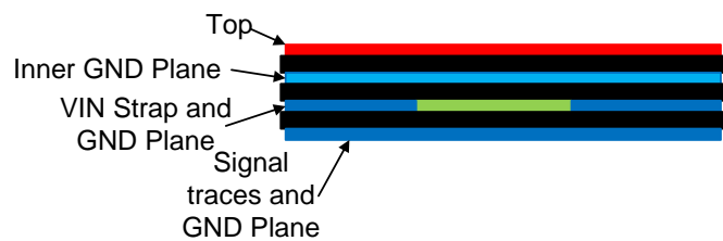
Figure 43. Example Layout
