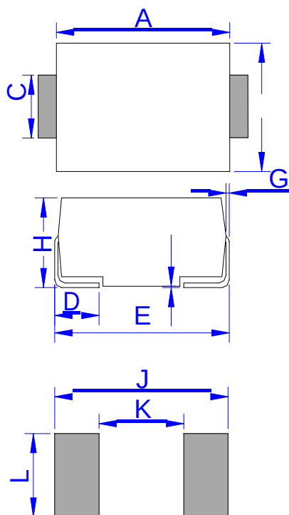
DO-214AA (SMB)
