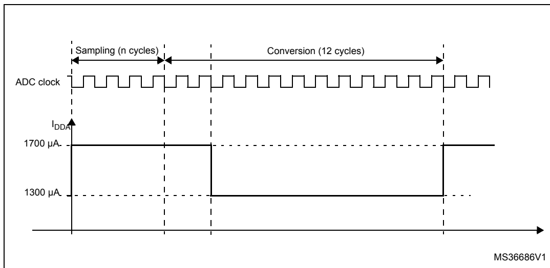
Figure 24. Maximum dynamic current consumption on V_{DDA} supply pin during ADC conversion
