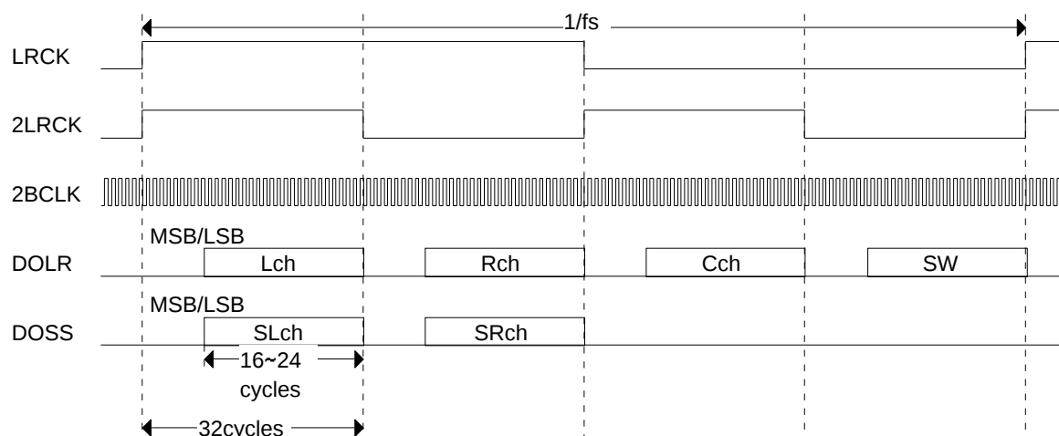
Figure 5.9 Right-justified Format Interface Between M65863FP and DAC(dacform[0]=0)
