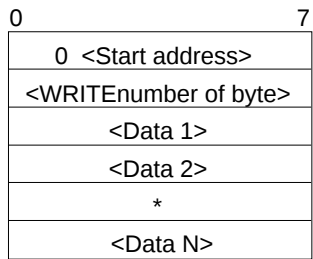
Figure 5.23 Instruction of Writing Registers of M65863FP
