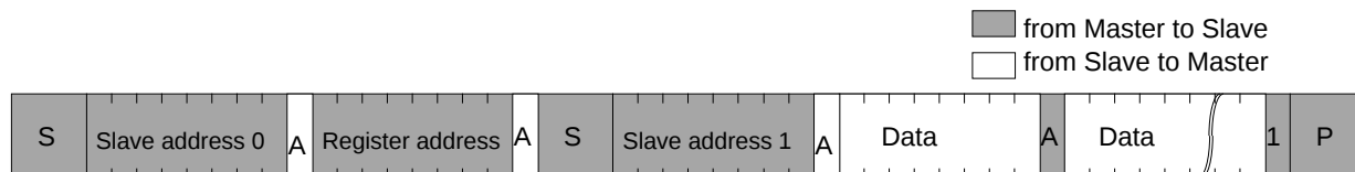
Figure 5.16 Master reads from M65863FP(slave) Register
