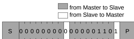
Figure 5.18 General Call Packet to Reset the M65863FP
