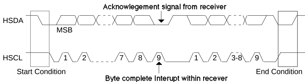
Figure 5.13 Data Transfer on the I 2 C BUS
