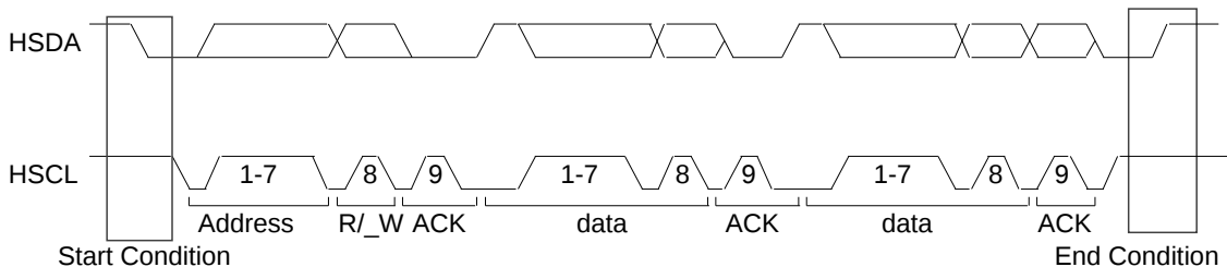
Figure 5.14 Data Transfer (7 bit address)
