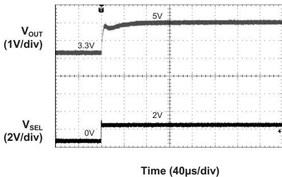
3.3V to 5V Transition Response ( I_{OUT} = 500mA , C_{OUT} = 10μF )
