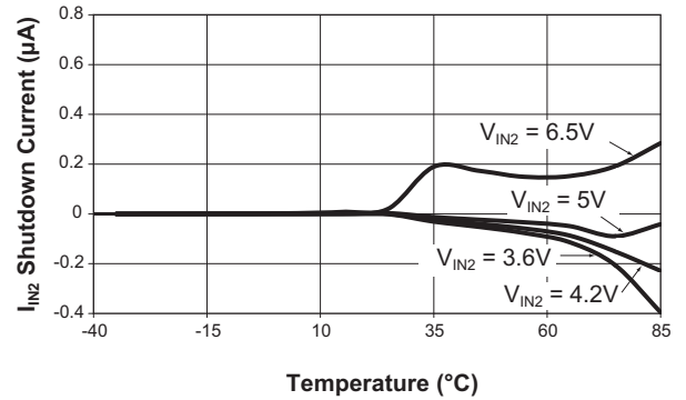
I_{IN2} Shutdown Current vs. Temperature
