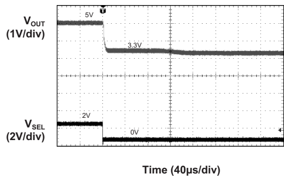
5V to 3.3V Transition Response ( I_{OUT} = 500mA , C_{OUT} = 10μF )
