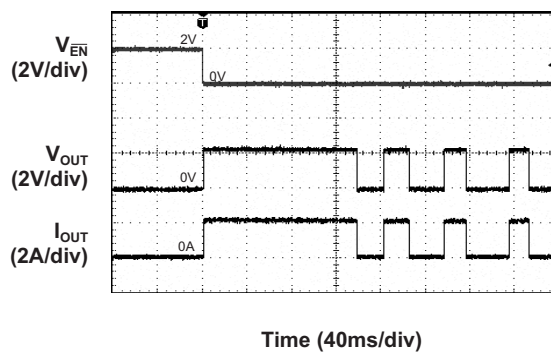
Thermal Shutdown Response (V_{IN} = 5\text{V})
