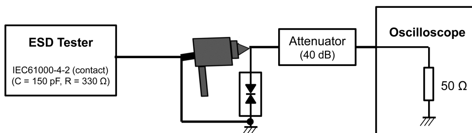
Fig. 10.3 IEC61000-4-2 (Contact)
