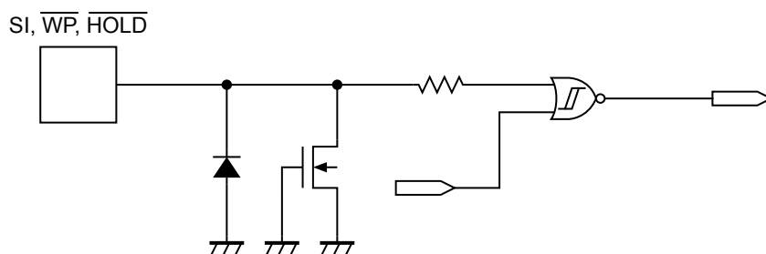
Figure 21 SI, WP, HOLD Pin
