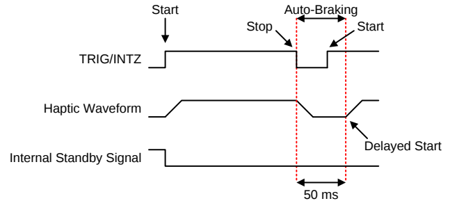
图 37. Trigger-Level with Delayed Start (RTP or Waveform Sequencer)
