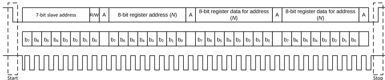
图 23. Typical I²C Sequence
