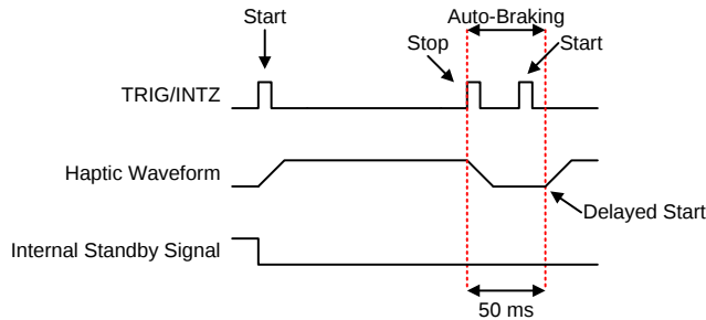
图 38. Trigger-Pulse and Delayed Start (RTP or Waveform Sequencer)
