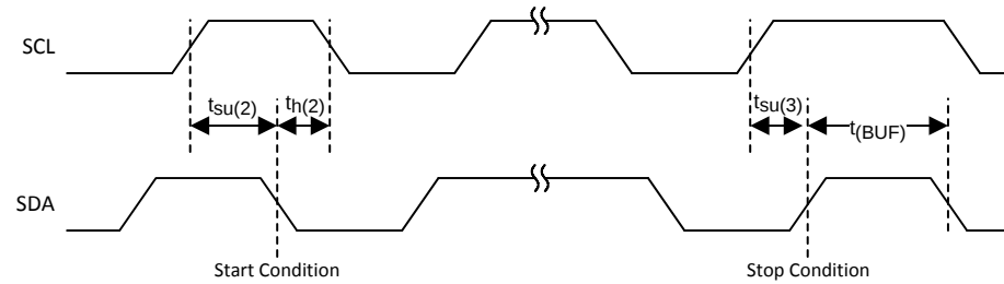
图 2. Timing for Start and Stop Conditions
