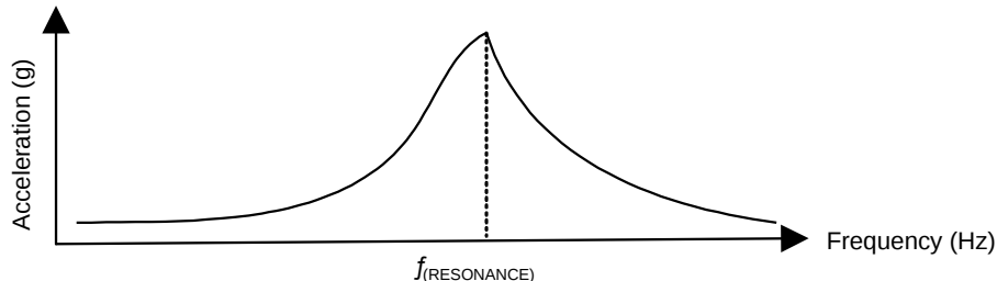
图 94. Typical LRA Response
