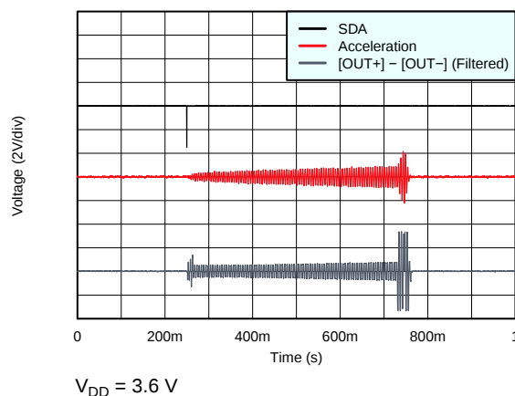
Figure 8. LRA Transition Click (Closed-Loop) with Internal Trigger
