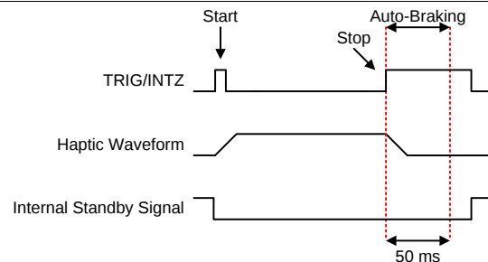
图 41. Trigger-Pulse Behavior when TRIG/INTZ Pin Left High (RTP or Waveform Sequencer)
