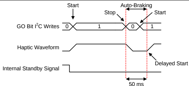
图 40. GO bit Trigger with Delayed Start (RTP or Waveform Sequencer)
