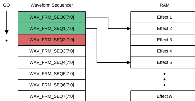
图 29. Waveform Sequencer Programming
