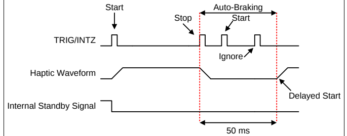
图 39. Trigger-Pulse and Delayed Start with Ignored Pulse (RTP or Waveform Sequencer)
