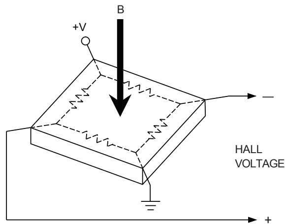
Dwg. AH-011-2
