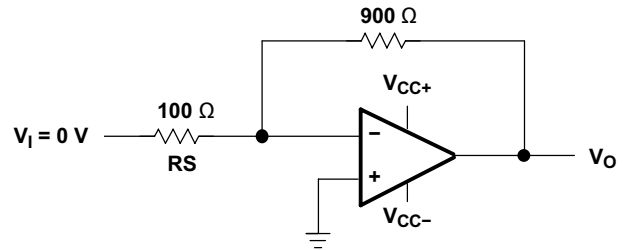
Figure 50. Noise-Test Circuit
