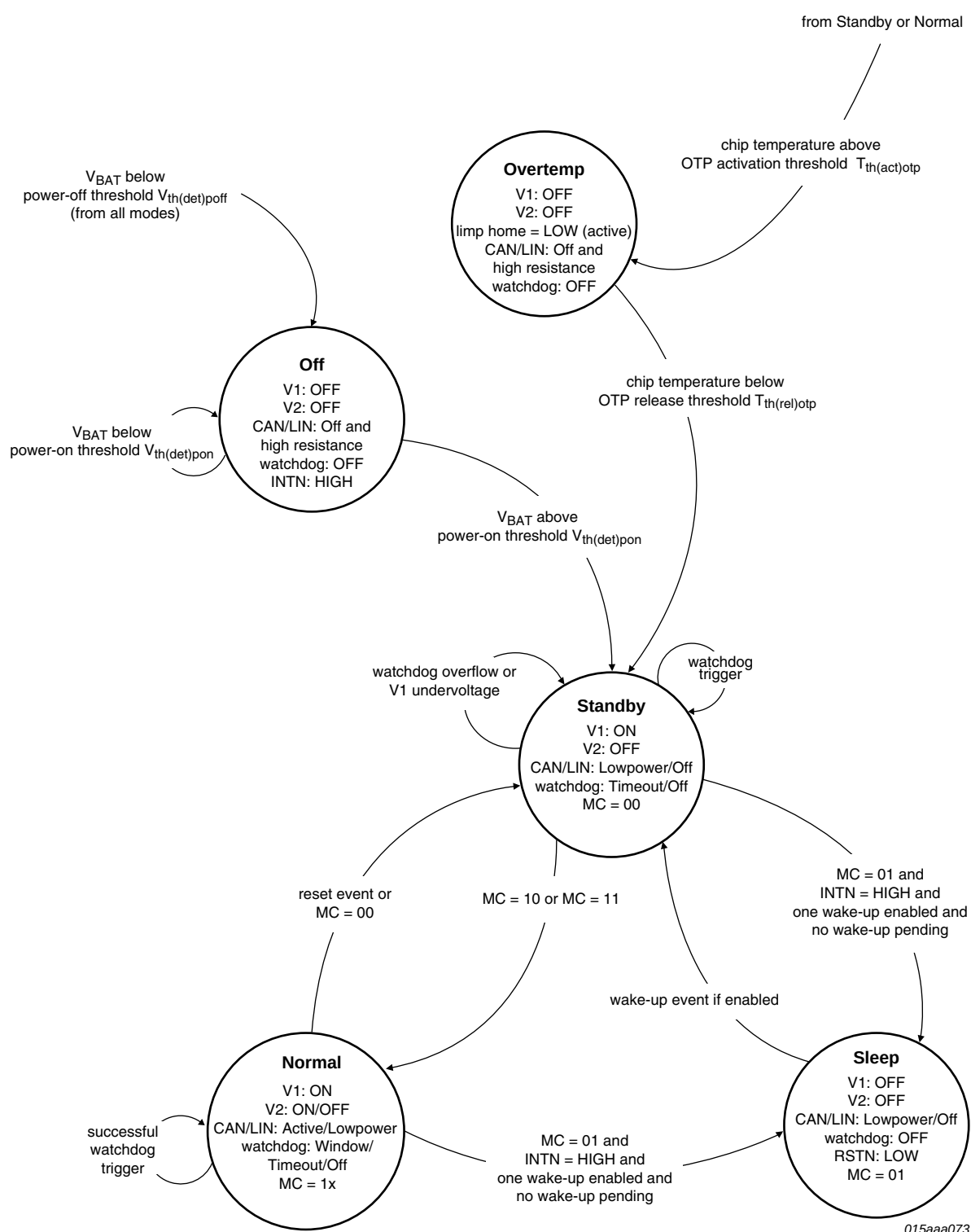
Fig 3. UJA1075A system controller
