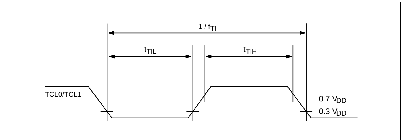
Figure 15-7. TCL0/TCL1 Timing
