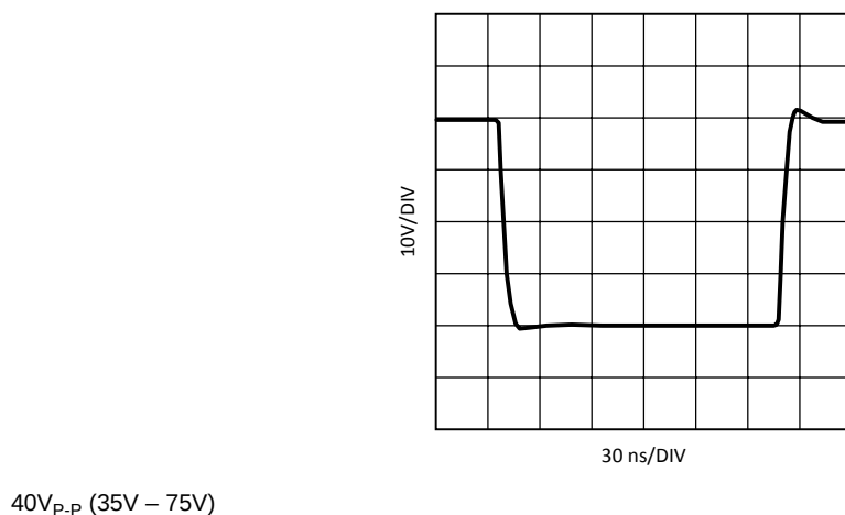
Figure 12. Typical Cathode Response
