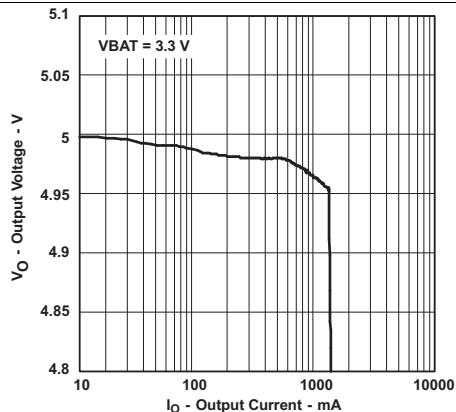
Figure 9. TPS61092 Output Voltage vs Output Current
