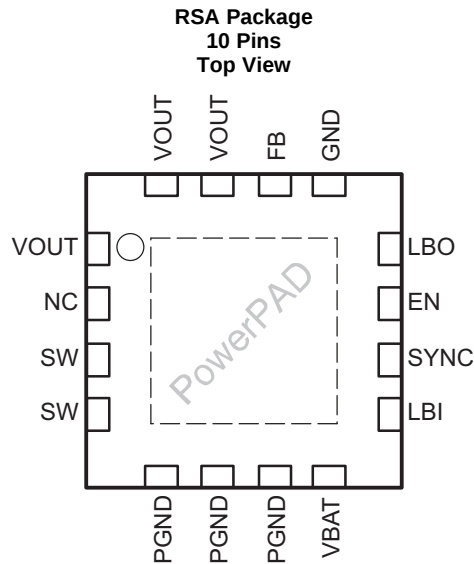
Pin Functions
