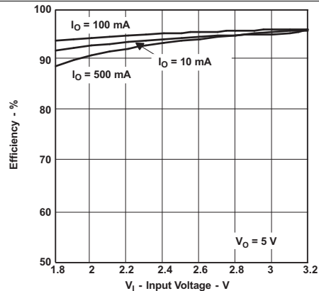
Figure 6. TPS61091 Efficiency vs Output Current
