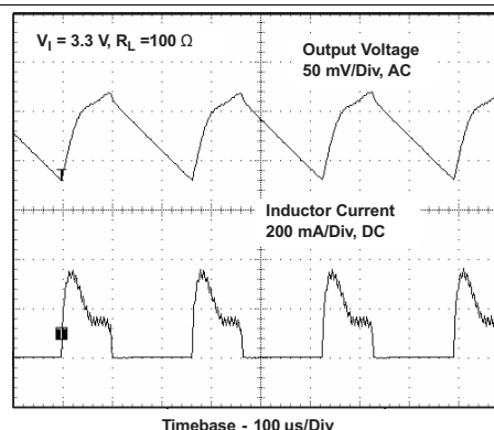
Figure 16. Output Voltage in Power Save Mode
