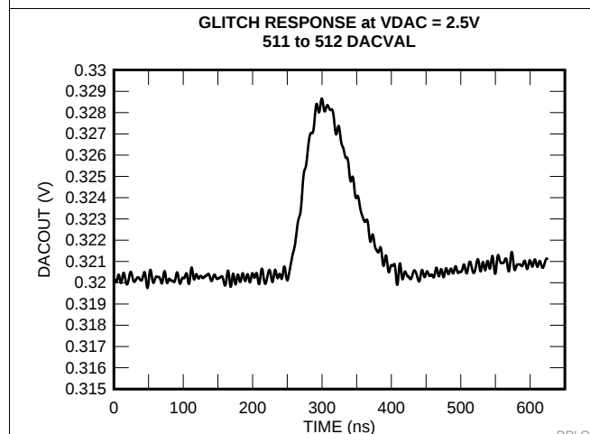
图 5-44. Glitch Response – 511 to 512 DACVAL
