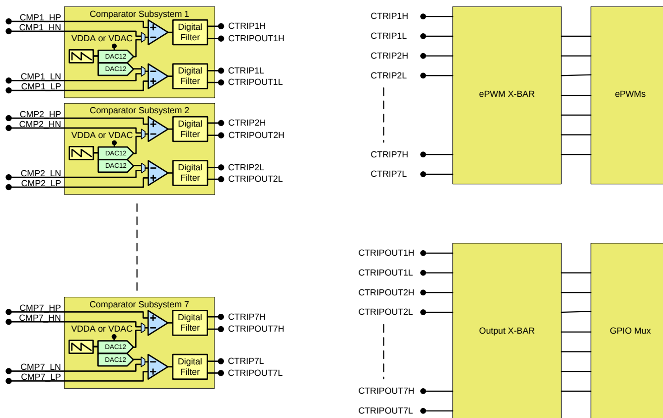
图 5-48. CMPSS Connectivity
