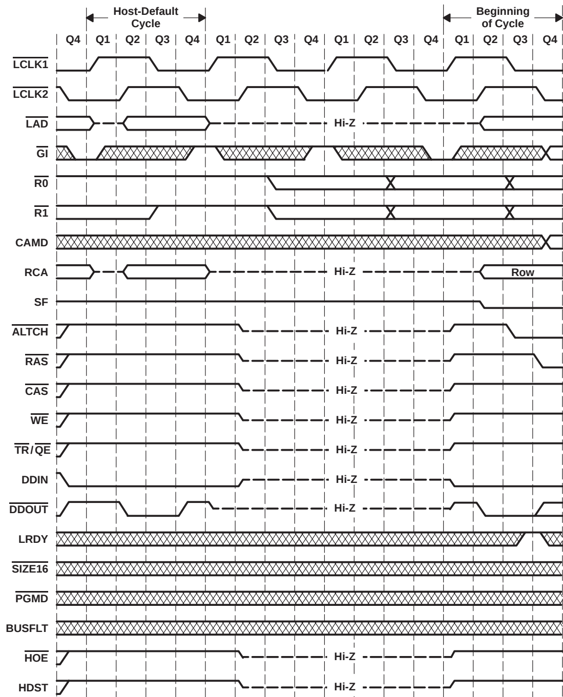
Figure 25. Multiprocessor-Interface-Cycle Timing (High-Impedance Signals)
