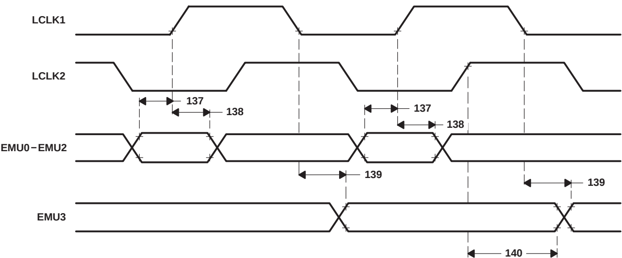
Figure 58. Emulator-Interface Timing
