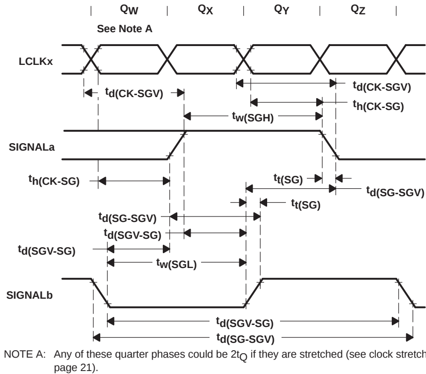
Figure 42. Output Signal Characteristics
