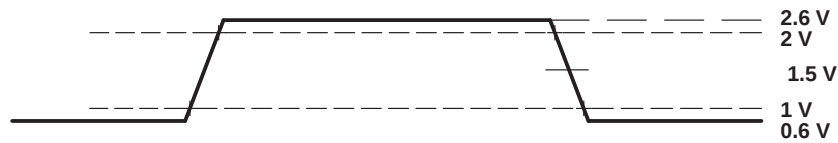
Figure 38. TTL-Level Outputs
