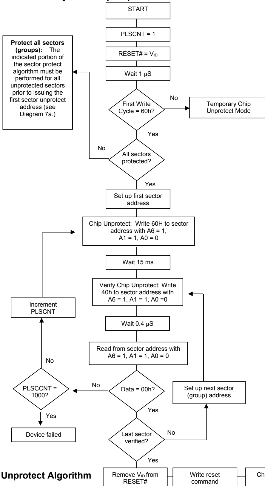
Flowchart 7b. In-System Chip Unprotect Flowchart
