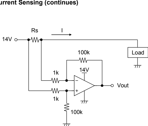
Figure6. High-Side Current Sensing
