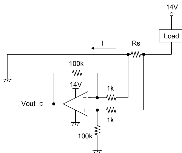
Figure7. Low-Side Current Sensing
