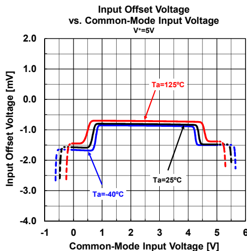
Figure2. Offset Voltage change with common-mode input voltage.
