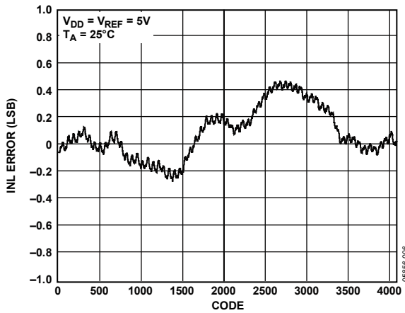
Figure 7. AD5624R INL, External Reference
