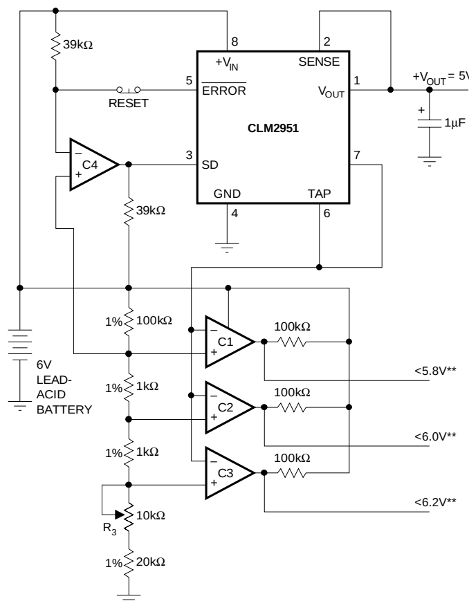
REGULATOR WITH STATE-OF-CHARGE INDICATOR
