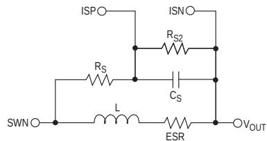
Figure 20: Current Sensing
