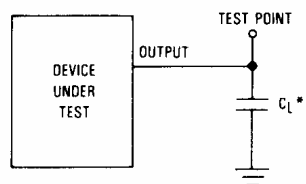
Figure 3. Test Circuit
