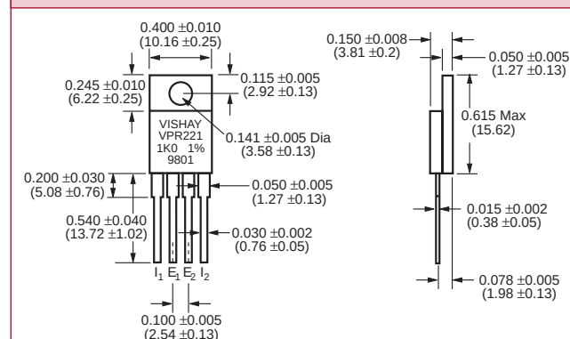
FIGURE 2 - VPR221 DIMENSIONS
