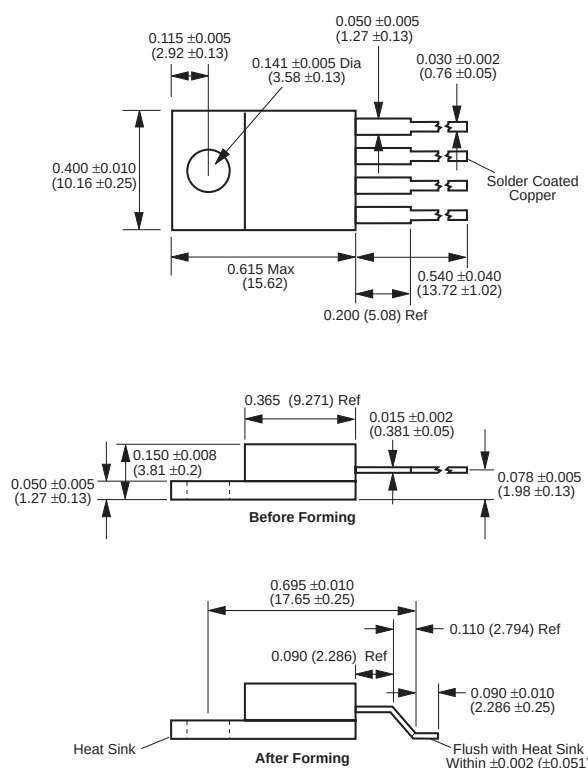
FIGURE 3 - VPR221S DIMENSIONS
