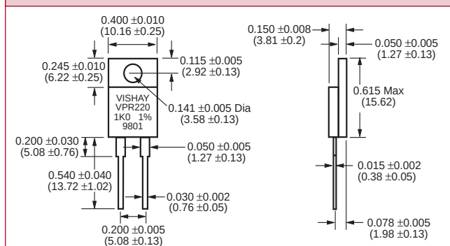
FIGURE 1 - VPR220 DIMENSIONS
