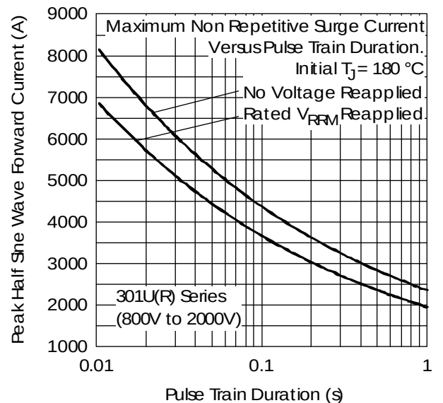
Fig. 10 - Maximum Non-Repetitive Surge Current
