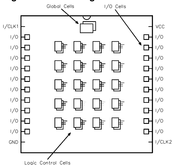
Figure 2: Block Diagram
