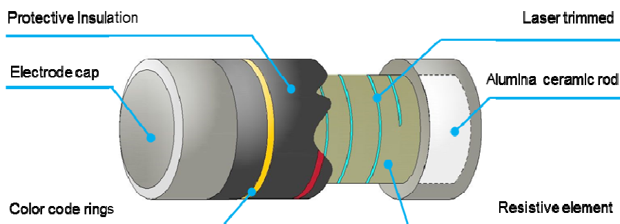
Fig 1. Construction of MELF
