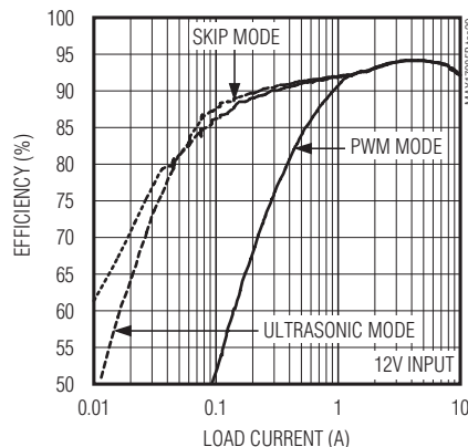
SMPS3 EFFICIENCY vs. LOAD CURRENT (CHARGER AND SMPS5 ARE OFF)
