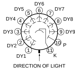
BOTTOM VIEW (BASING DIAGRAM)
