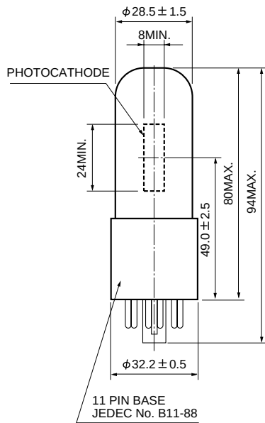
Figure 8: Dimensional Outline and Basing Diagram(Unit: mm) Figure 10: Socket E678-11A (Option)
